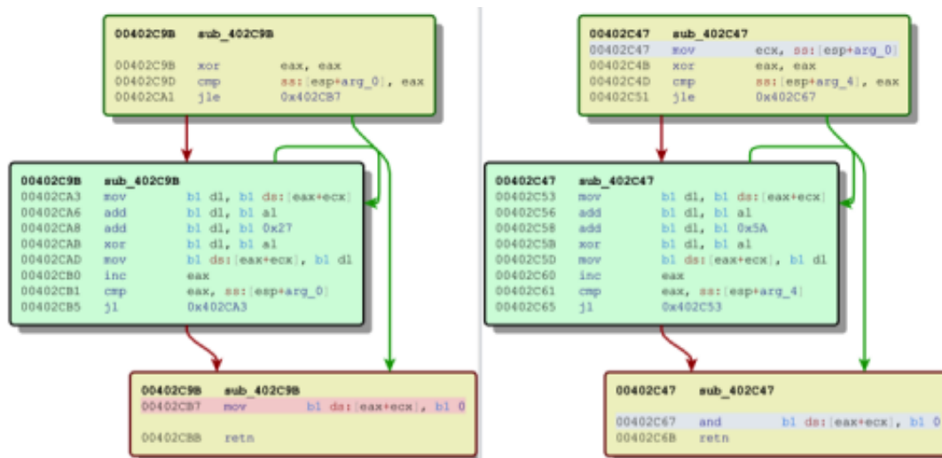
Figure 3. Comparing a BS2005 and post Ke3chang sample C2 obfuscation routine
